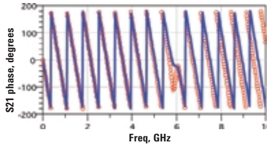
Figure 34. ADS model of the nine inch long trace, modeling the coupling to the adjacent, quiet line, showing the bandwidth of the model to be ~8 GHz.
