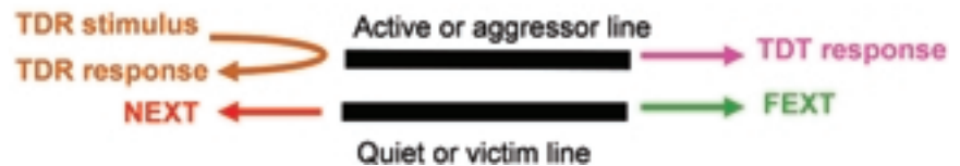
Figure 36. Configuration for two-port TDR measurements.
