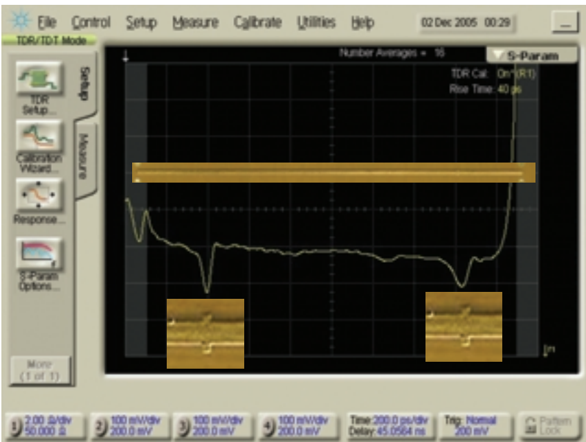
Figure 9. TDR response of a uniform transmission line with two small reference pads, located on four inch centers.
