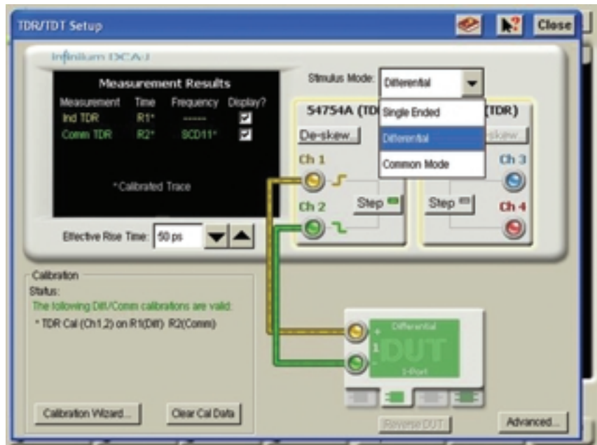
Figure 50. DTDR set up screen for differential measurements.
